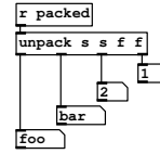
fig 3.17: List unpacking
