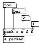
fig 3.16: List packing
