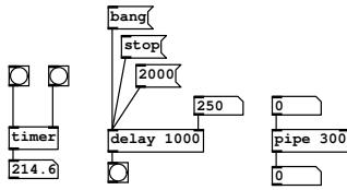
fig 3.8: Time objects
