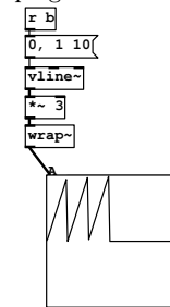
fig 6.13: Wrapping a line
