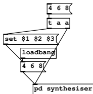
fig 3.19: Persistence using messages
