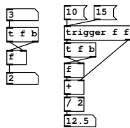
fig 3.38: Last value and averaging
