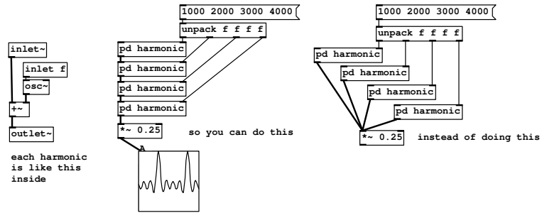
fig 5.18: Stacking subpatches that sum with an inlet
