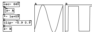
fig 6.7: Square wave
