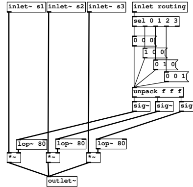
fig 7.13: demultiplex
